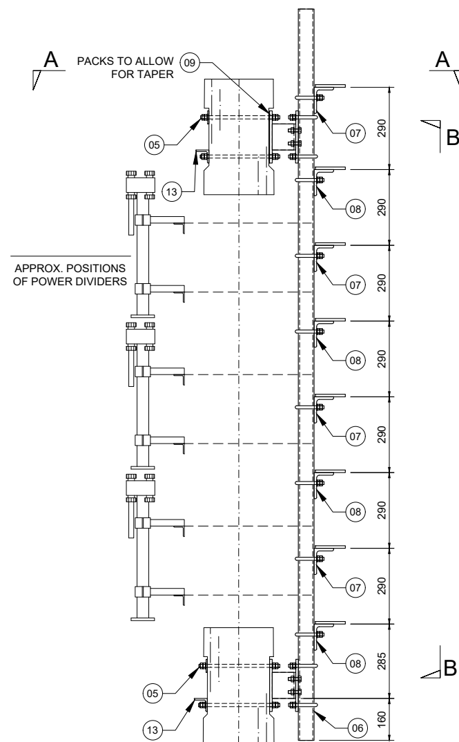
DETAIL G - Tx ANTENNA MOUNT Scale 1:20
