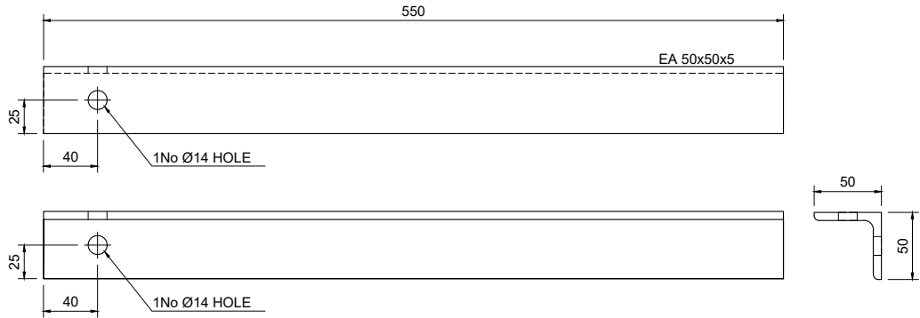
TPA-BR-1 - EA50x50x5 Scale 1:5
